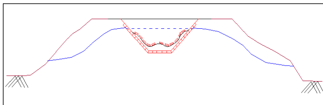
Figure 5. Disturbed Profile of Canal Due to Swelling of Embankment Soil
