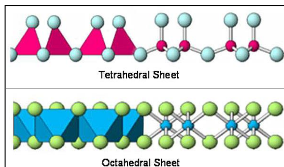
Figure 1. Silicon Tetrahedron sheets and Aluminum Octahedral sheets
