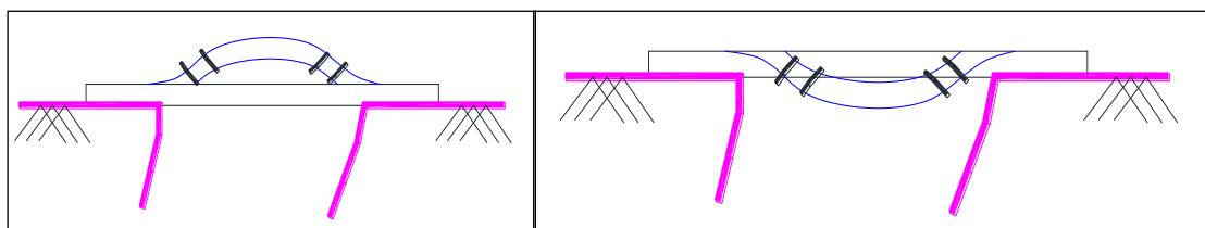
Figure 6. Hogging and sagging of lining due to cyclical swelling and shrinkage
