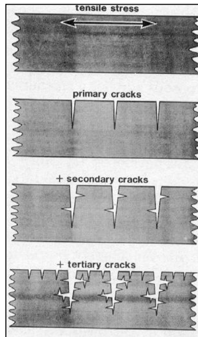
Figure 4. Formation of cracks due to shrinkage preceded by swelling (Dexter 1988)
